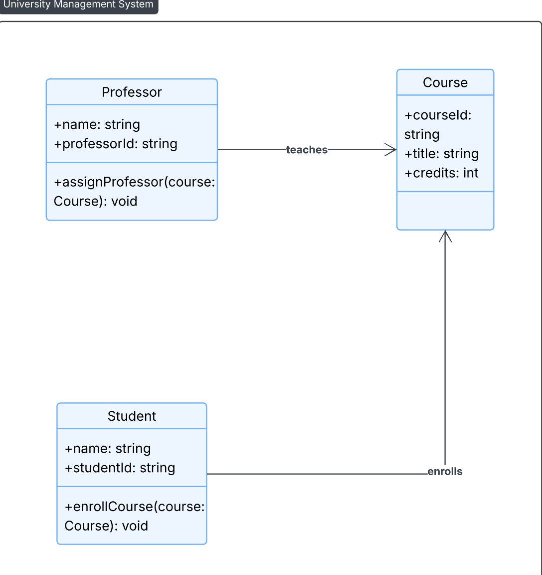
University Management System
