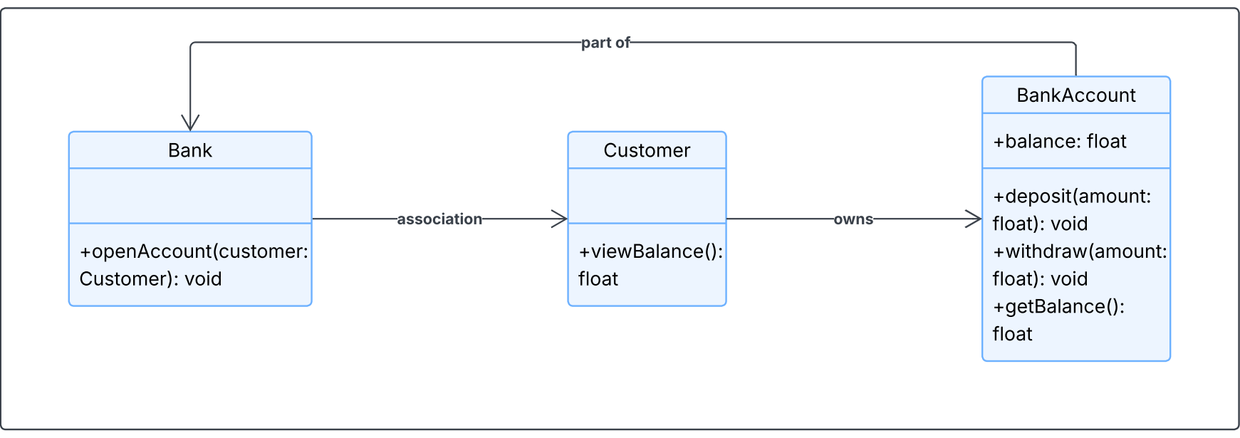
Bank and Customer Association Relationship Diagram
