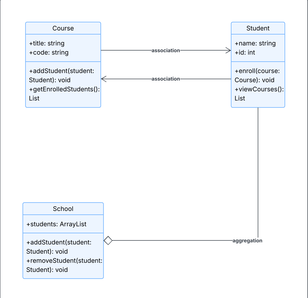
School, Students, and Courses (Association and Aggregation)
