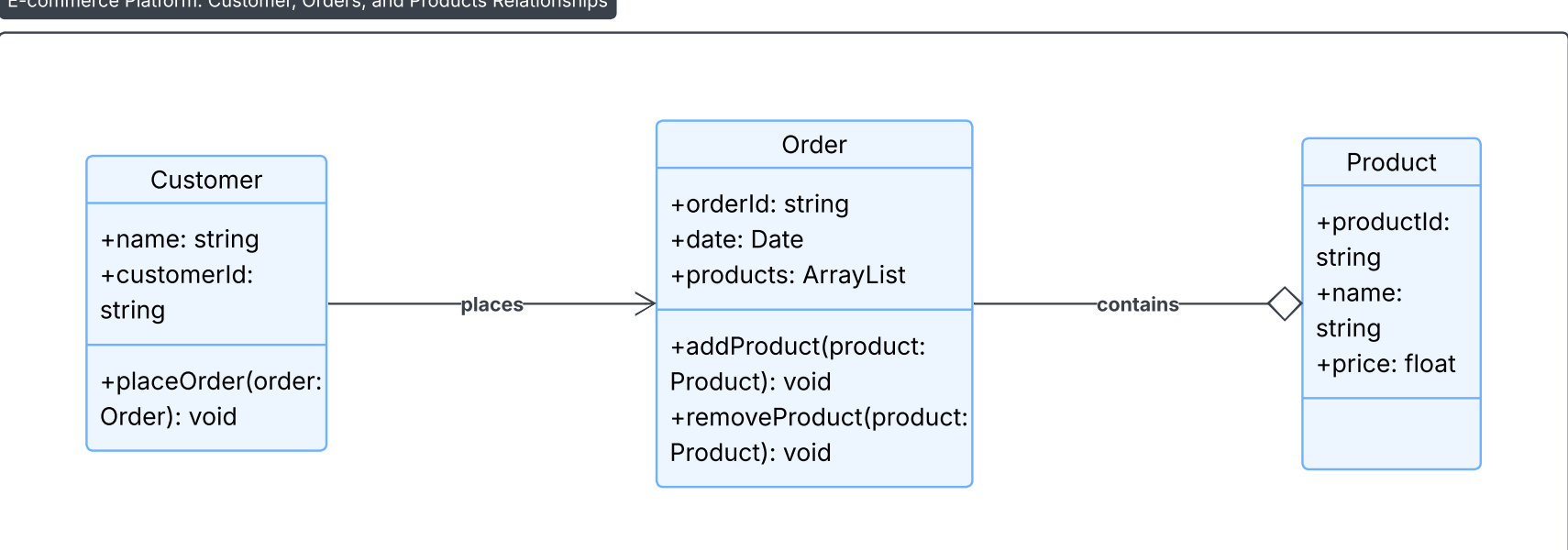
E-commerce Platform: Customer, Orders, and Products Relationships
