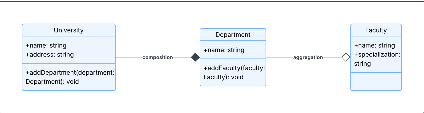
University Composition and Aggregation with Faculties and Departments
