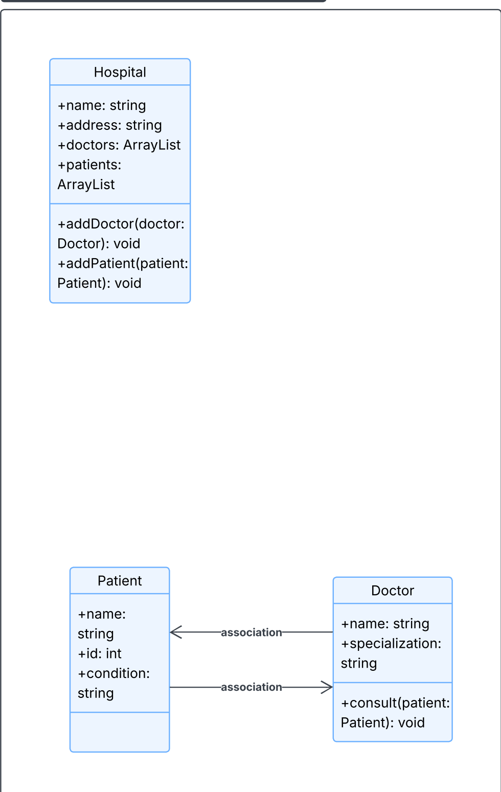
Hospital, Doctors, and Patients (Association and Communication)
