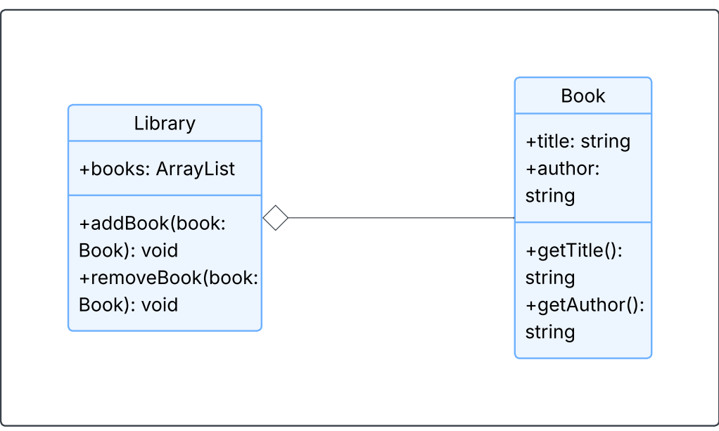
Library and Books Aggregation Model
