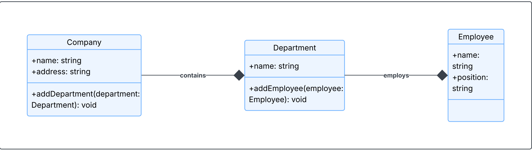
Company and Departments (Composition)
